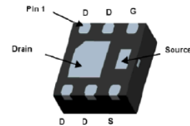
DFN2X2-6L bottom view
