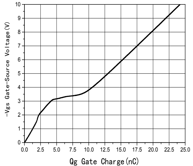
Fig6 Gate Charge
