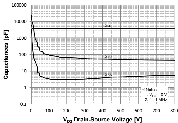
Figure 5. Capacitance Characteristics
